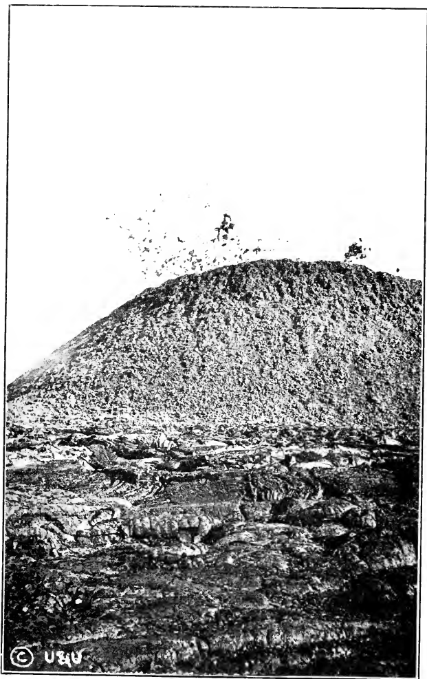
MOKUAWEOWEO. MAUNA LOA, IN ERUPTION, 1899
